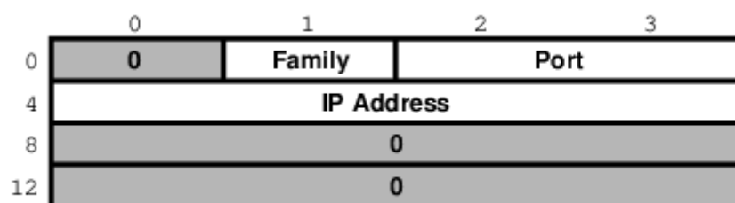
Figure 3. sockaddr_in structure
